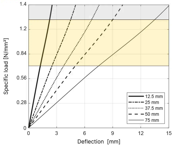
T100 Load deflection - Shape factor 3.0
