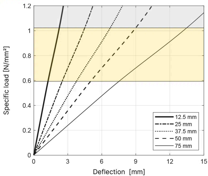
T100 Load deflection - Shape factor 1.5
