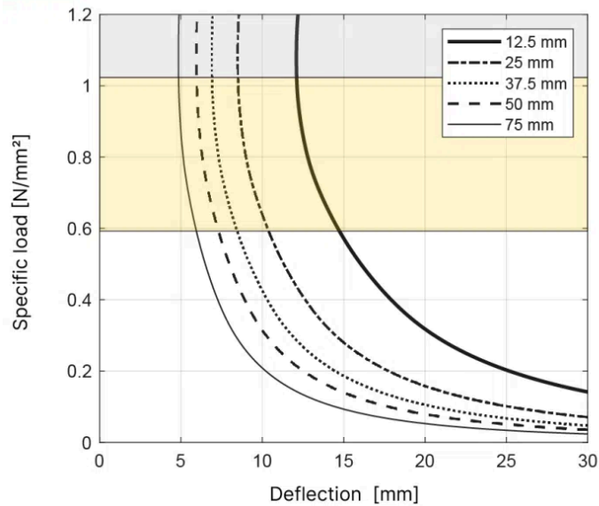
T100 Natural frequency - Shape factor 1.5
