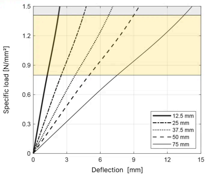
T100 Load deflection - Shape factor 6.0
