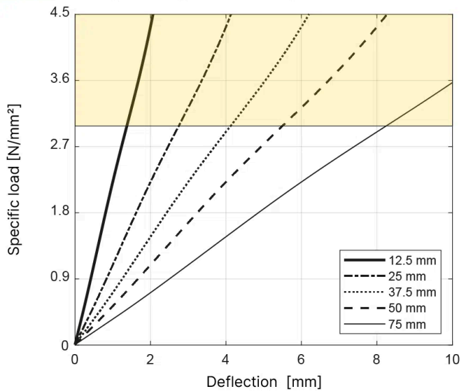
T300 Load deflection - Shape factor 3.0
