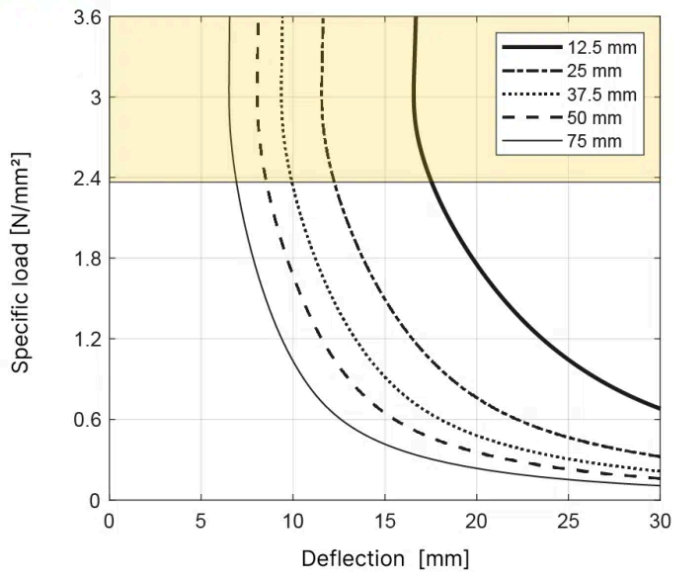
T300 Natural frequency - Shape factor 1.5
