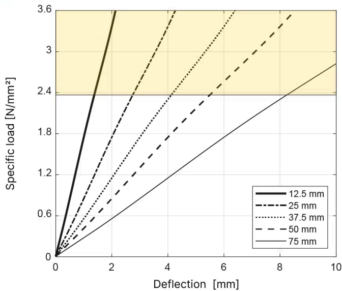
T300 Load deflection - Shape factor 1.5
