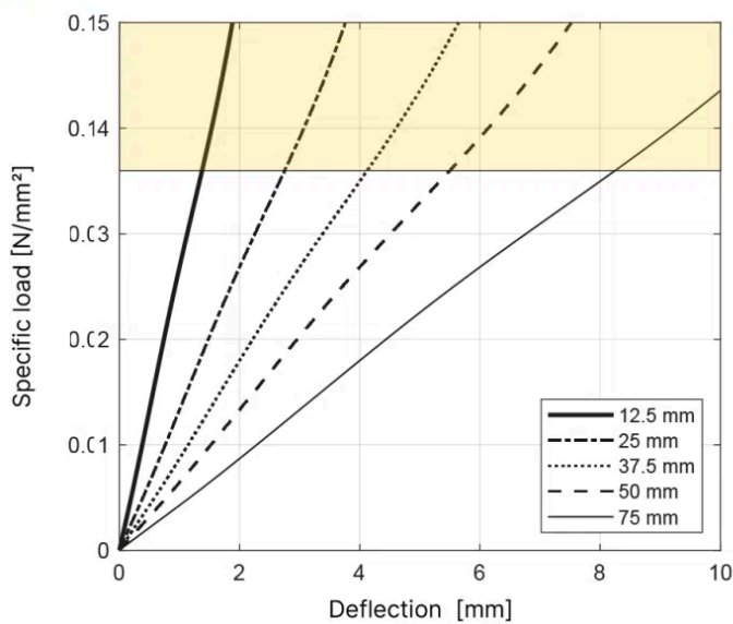
T300 Load deflection - Shape factor 6.0
