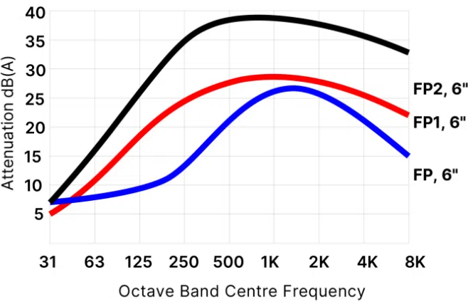
Typical Attenuation Curve
