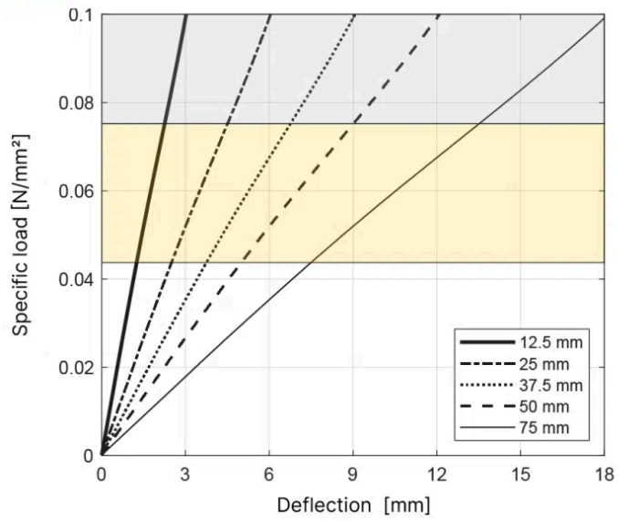
T006 Load deflection - Shape factor 1.5
