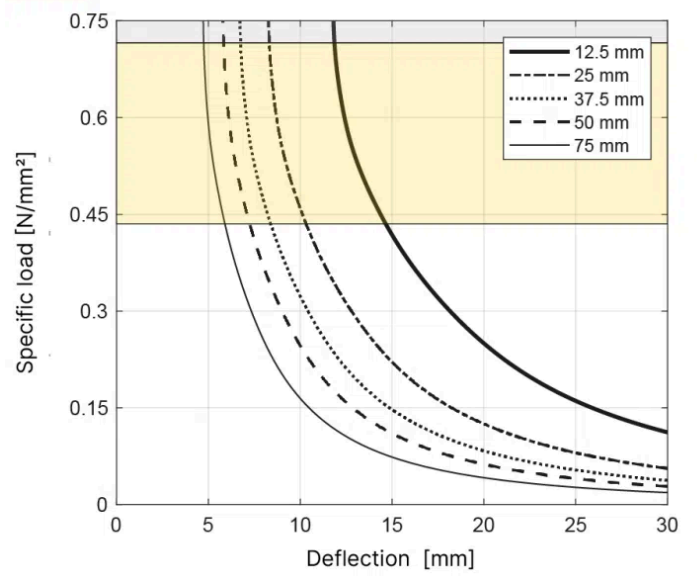
T060 Natural frequency - Shape factor 6.0
