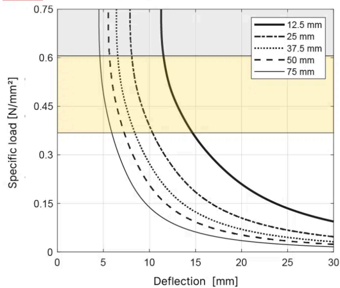
T060 Natural frequency - Shape factor 1.5
