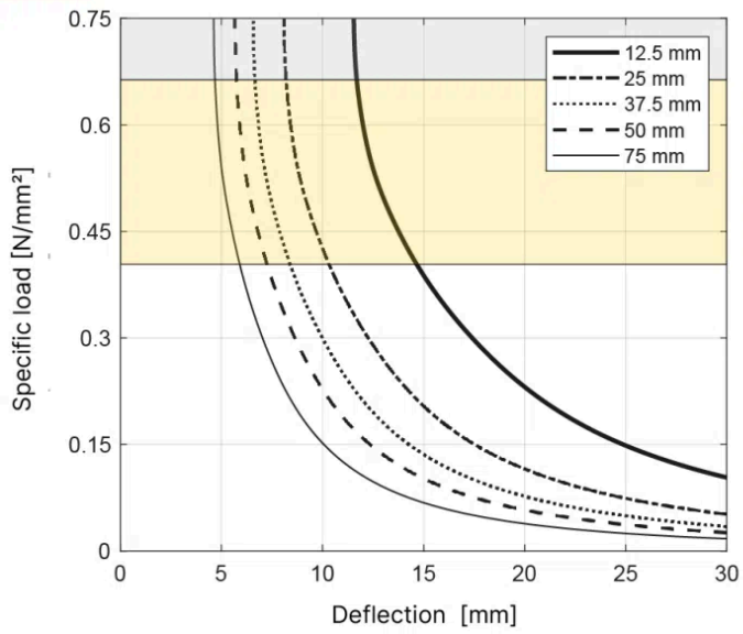
T060 Natural frequency - Shape factor 3.0
