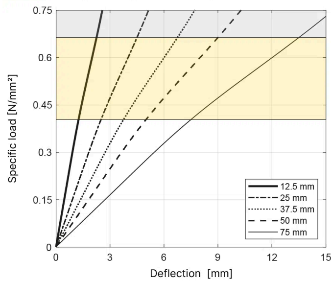
T060 Load deflection - Shape factor 3.0
