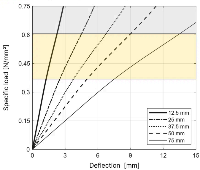
T060 Load deflection - Shape factor 1.5
