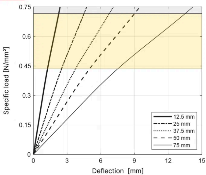
T060 Load deflection - Shape factor 6.0
