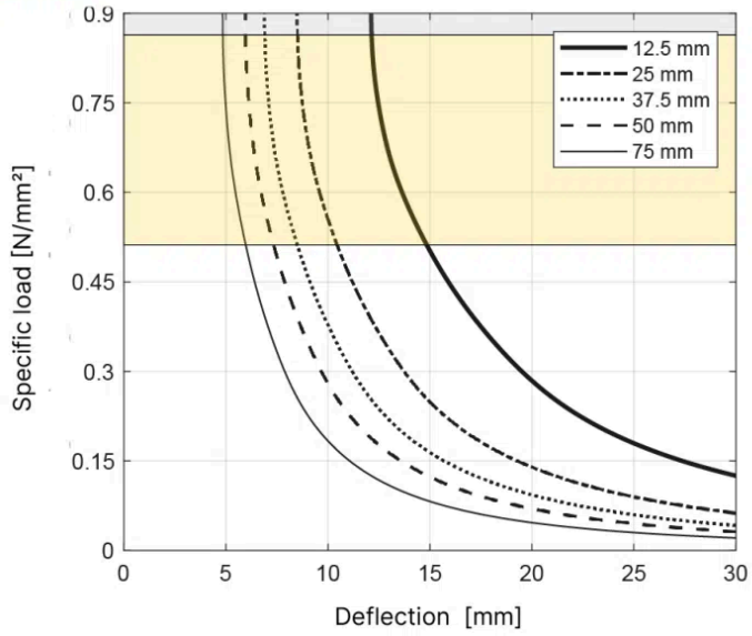
T075 Natural frequency - Shape factor 3.0
