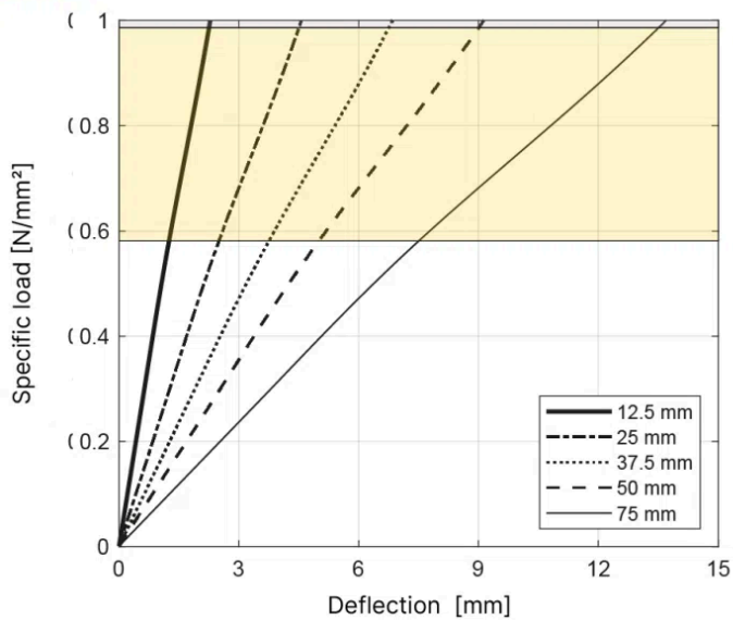
T075 Load deflection - Shape factor 6.0
