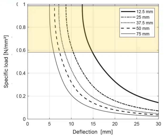
T075 Natural frequency - Shape factor 6.0
