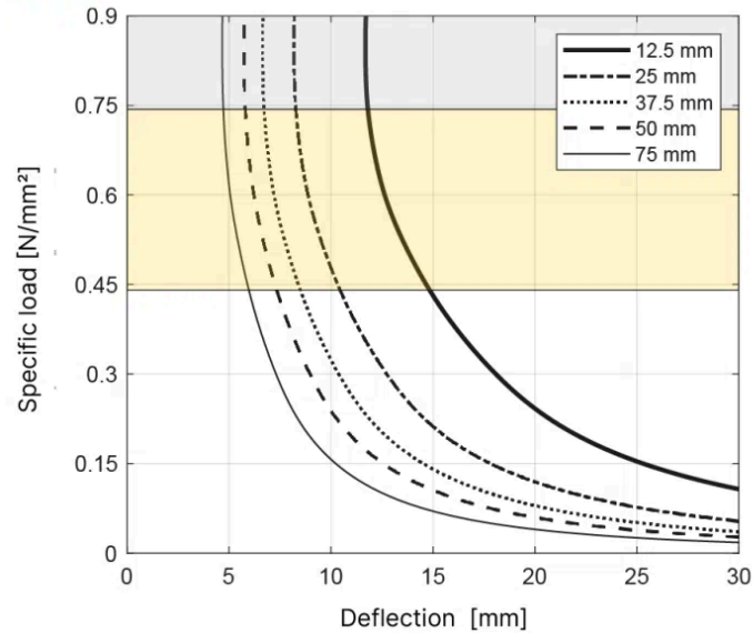
T075 Natural frequency - Shape factor 1.5
