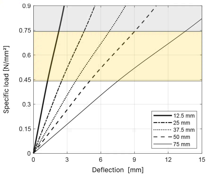
T075 Load deflection - Shape factor 1.5
