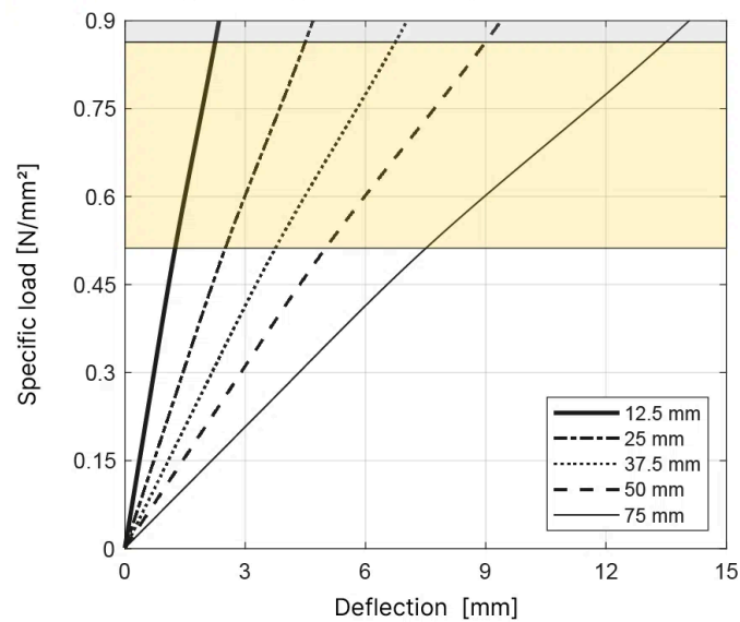
T075 Load deflection - Shape factor 3.0
