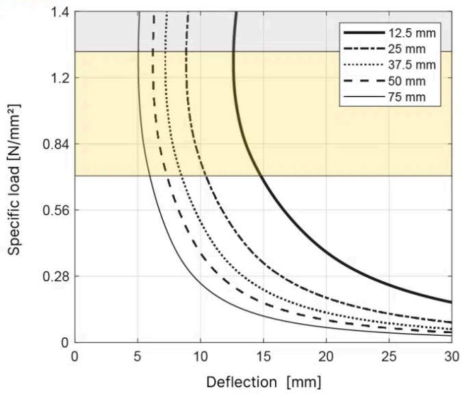
T100 Natural frequency - Shape factor 3.0
