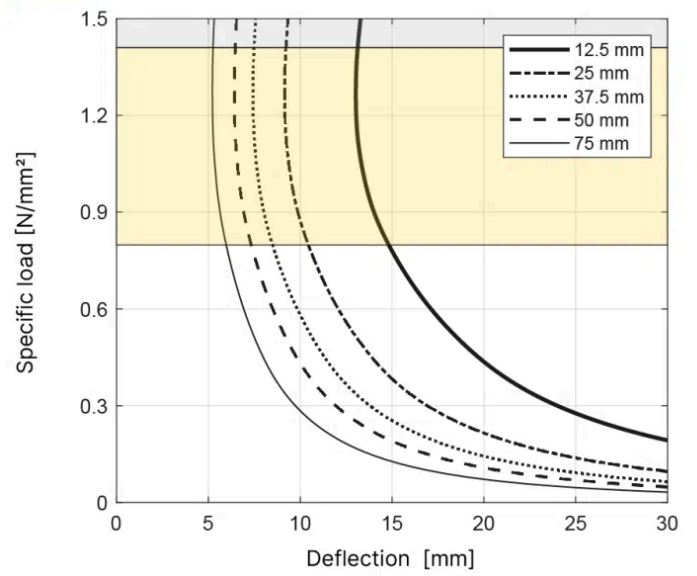
T100 Natural frequency - Shape factor 6.0
