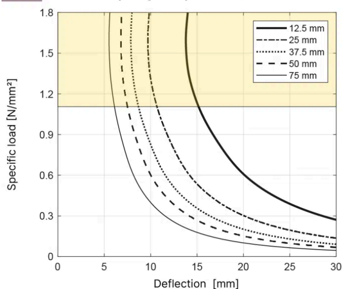
T125 Natural frequency - Shape factor 6.0
