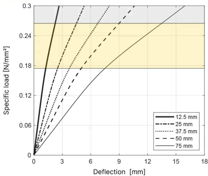
T018 Load deflection - Shape factor 6.0
