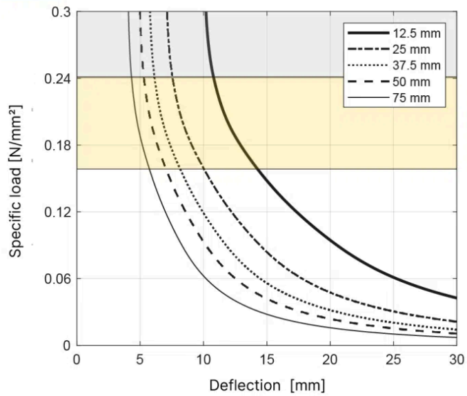
T018 Natural frequency - Shape factor 3.0
