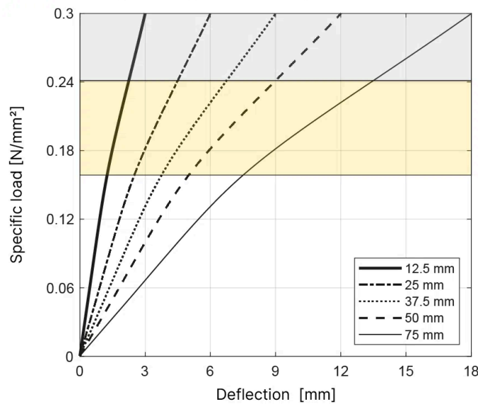
T018 Load deflection - Shape factor 3.0
