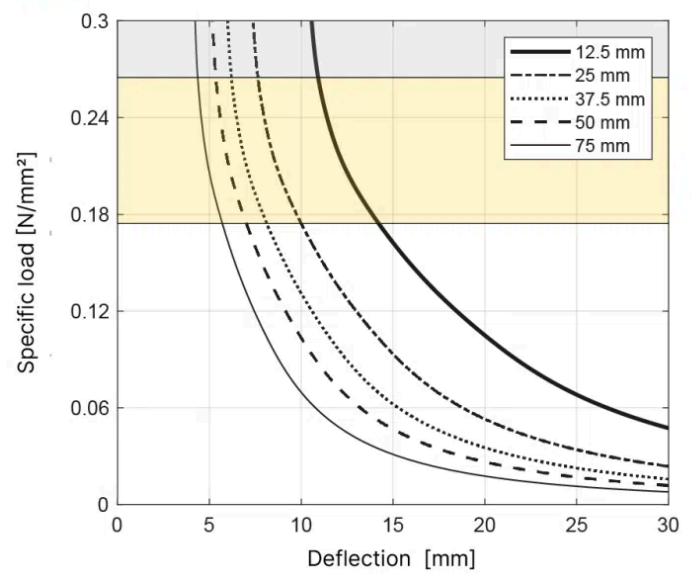
T018 Natural frequency - Shape factor 6.0
