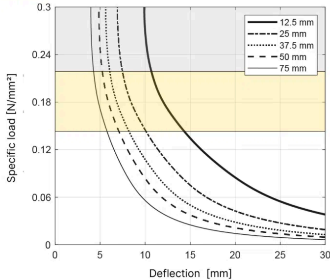
T018 Natural frequency - Shape factor 1.5
