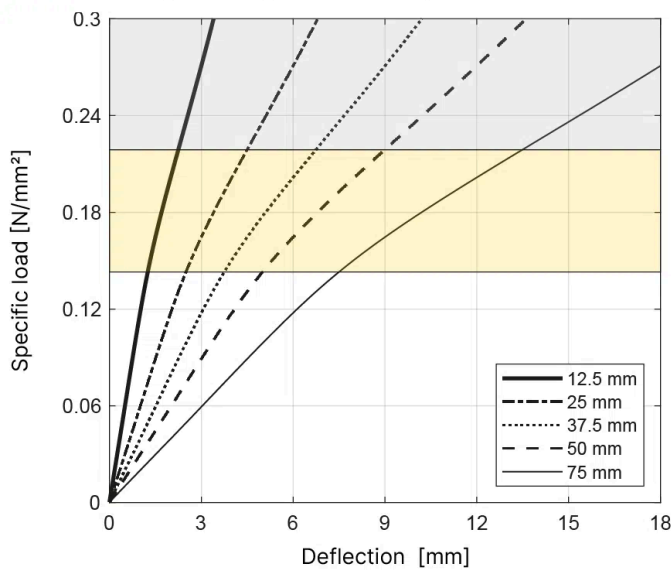
T018 Load deflection - Shape factor 1.5
