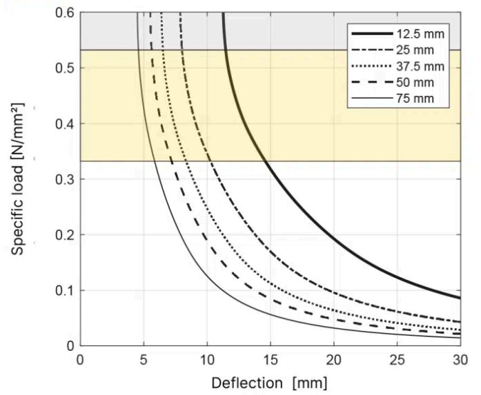
T045 Natural frequency - Shape factor 6.0
