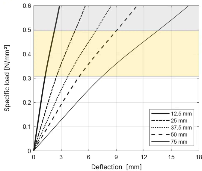
T045 Load deflection - Shape factor 3.0
