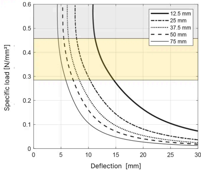
T045 Natural frequency - Shape factor 1.5
