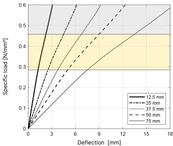
T045 Load deflection - Shape factor 1.5
