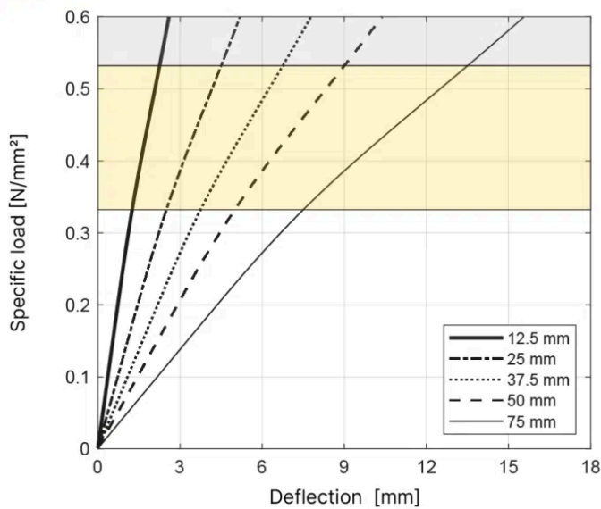
T045 Load deflection - Shape factor 6.0
