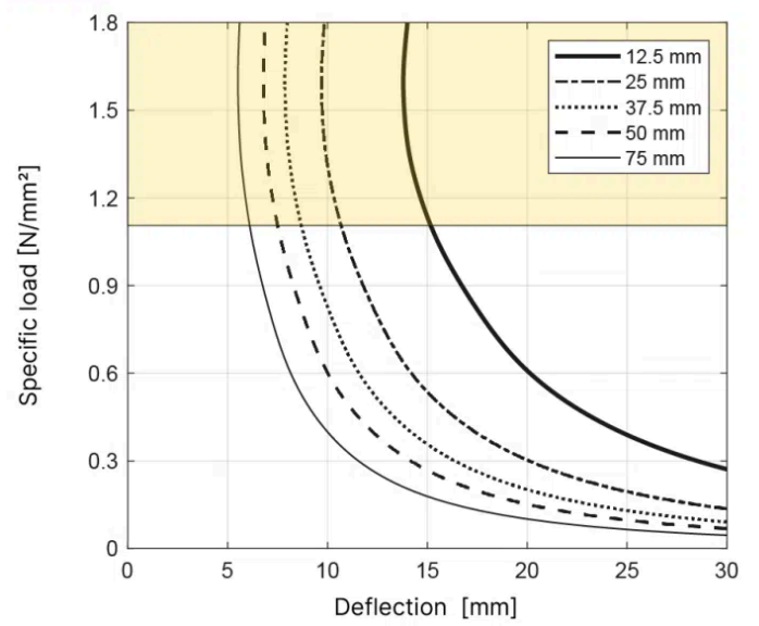
T125 Natural frequency - Shape factor 6.0
