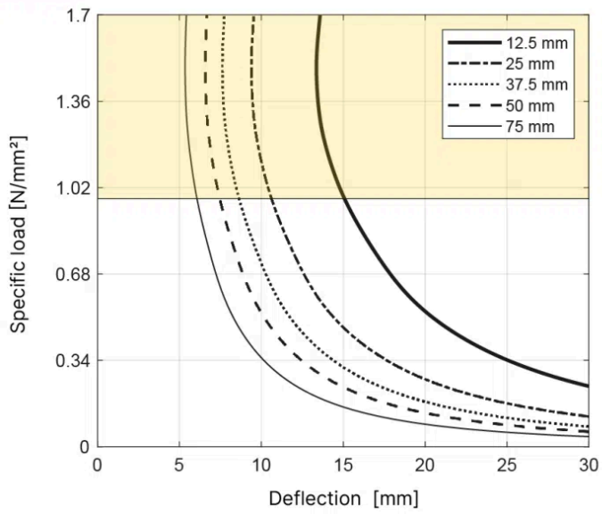
T125 Natural frequency - Shape factor 3.0
