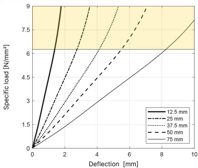
T600 Load deflection - Shape factor 3.0
