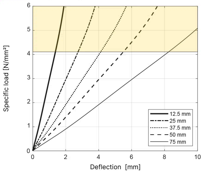
T600 Load deflection - Shape factor 1.5
