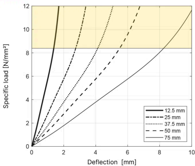
T600 Load deflection - Shape factor 6.0
