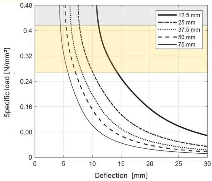
T035 Natural frequency - Shape factor 3.0
