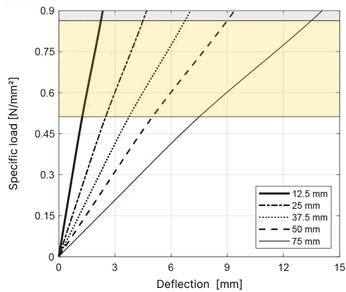
T075 Load deflection - Shape factor 3.0
