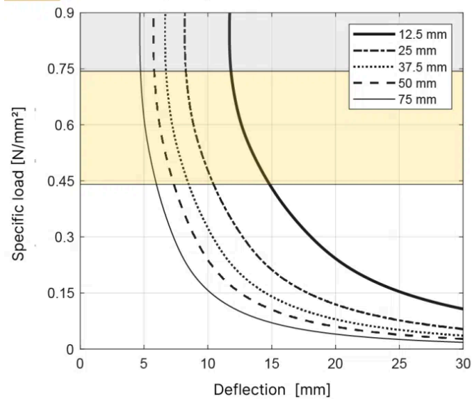
T075 Natural frequency - Shape factor 1.5
