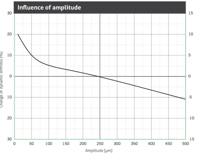
Change of the dynamic stiffness due to changes in amplitudes. Average for 5 Hz, 10 Hz and 40 Hz excitation. Sinusoidal excitation at a constant mean load of 0.011 N/mm 2 , dimensions of the specimens 300 x 300 x 25 mm. Natural frequency of a single-degree-of-freedom system (SDOF system) on a rigid base.
