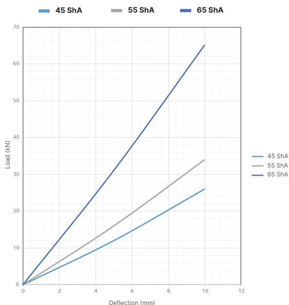
Load-Deflection HD Marine
