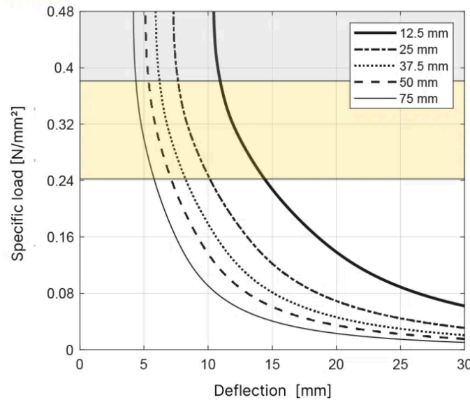
T035 Natural frequency - Shape factor 1.5
