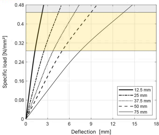
T035 Load deflection - Shape factor 6.0
