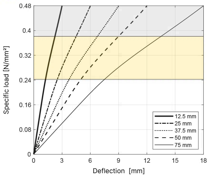
T035 Load deflection - Shape factor 1.5
