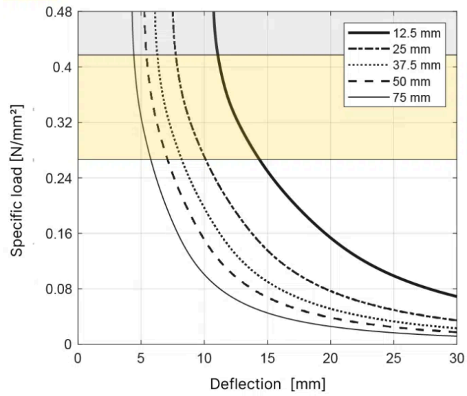
T035 Natural frequency - Shape factor 3.0
