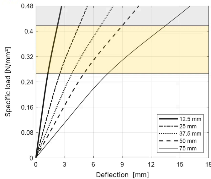
T035 Load deflection - Shape factor 3.0
