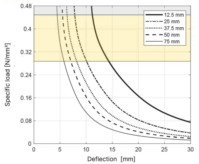
T035 Natural frequency - Shape factor 6.0
