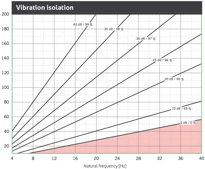
Illustration of the isolation efficiency of a single-degree-of-freedom system (SDOF system) on a rigid base with REGUFOAM vibration 150plus . Parameter: power transmission (insertion loss) in dB, isolation factor in %.
